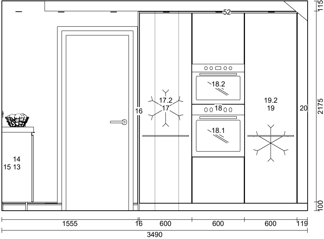
Elevation B/B
